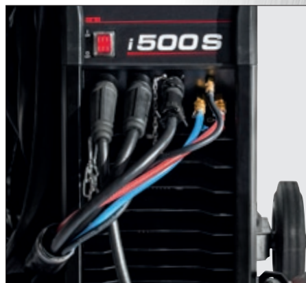
Cable connections on front (in standard) and back rear side (in option). Strain reliefs on both ends to keep connections well protected.
